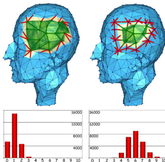
Figure 1: Geometry-driven coding with free valences (left) in practice yield a lower symbol dispersion than coding with full valences (right). The frequency of local and global splits is negligibly low for this particular model.
