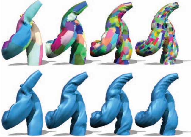
Figure 6: Constraint resolution . Increasing the number of partitions (left-to-right: 16, 64, 256, 1024) narrows the support of the test functions, forcing closer tracking and finer wrinkles.
